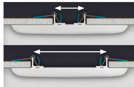
Surface mountable
